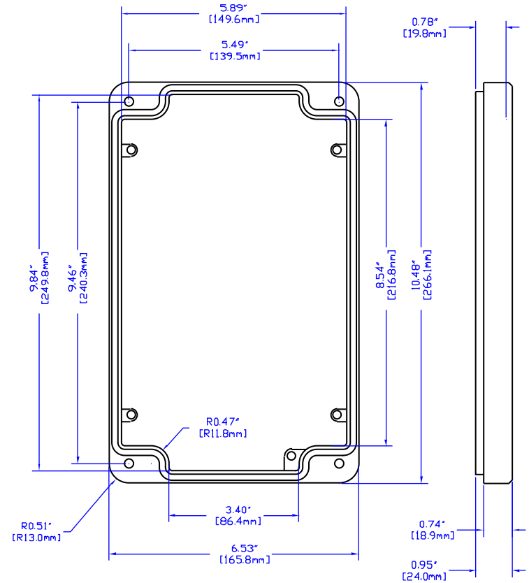
VIEW OF LID (INSIDE)
